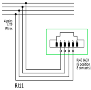
1G telephone outlet
