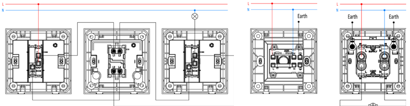
1G intermediate switch
