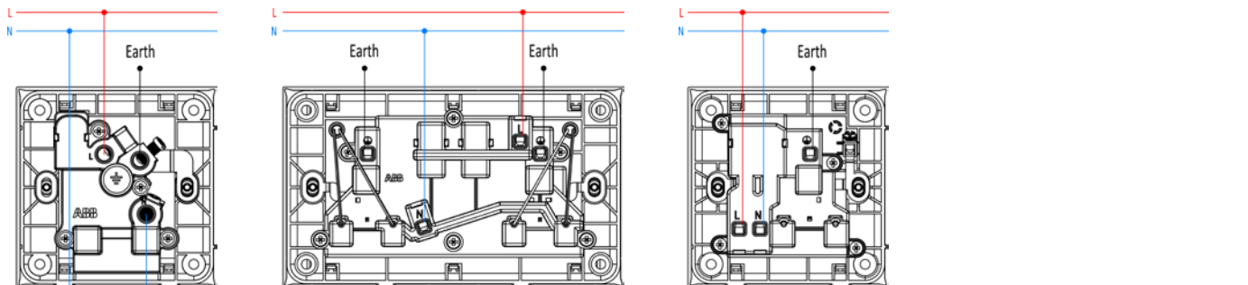
1G switch socket outlet
